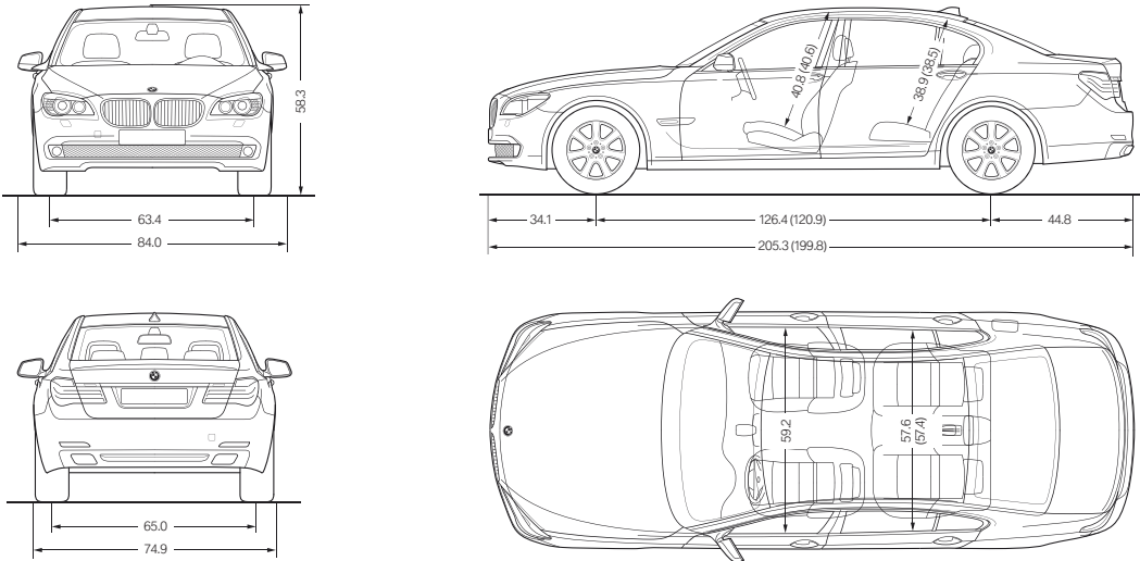
Technical drawings show 750Li, 750Li xDrive and 760Li with dimensions given in inches. Figures in ( ) refer to the 750i (short-wheelbase version). Height of 750Li and 750Li xDrive with roof antenna is 58.5 inches; 750i and 750i xDrive height with roof antenna is 58.7 inches.
