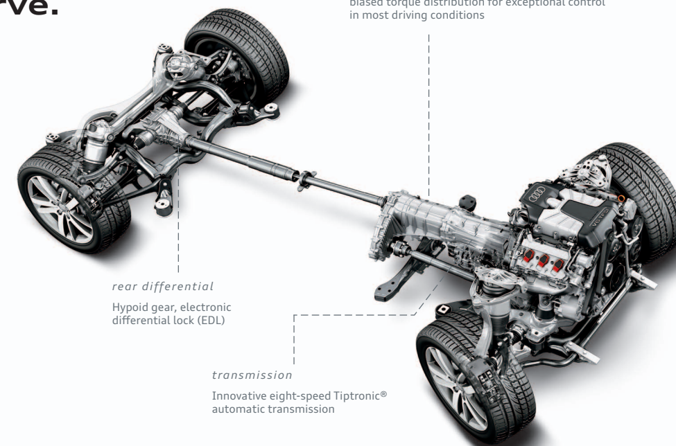
torque-sensing center differential
