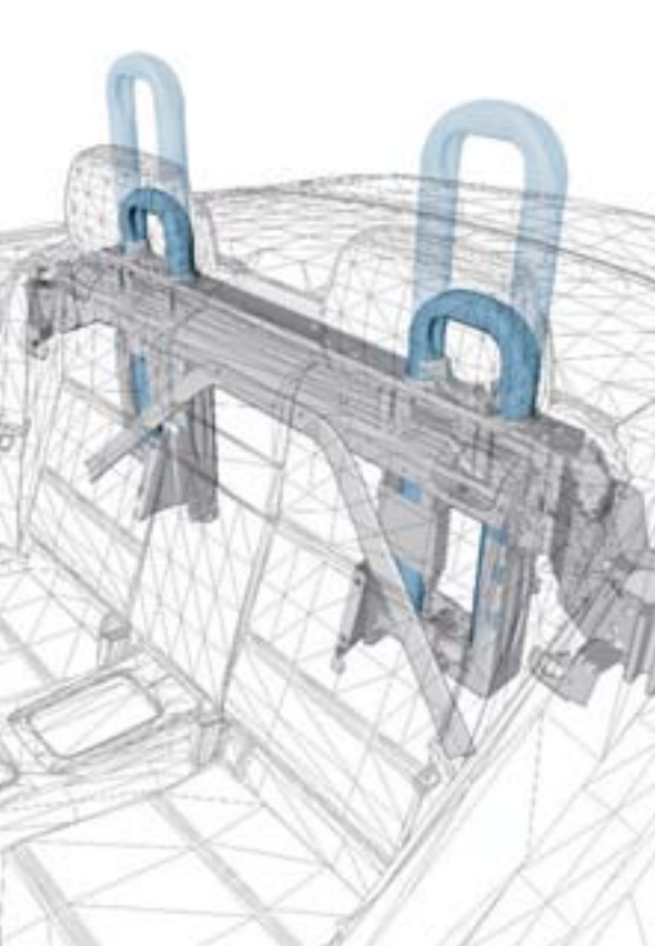
In the event of a rollover, sensors ensure that the rollover bars are deployed within fractions of a second.
