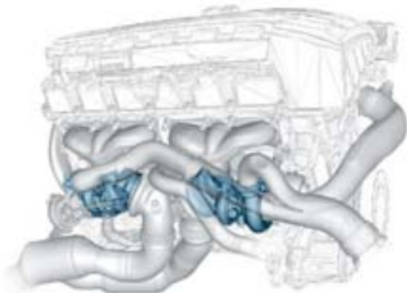
Fast buildup of pressure: the two parallel turbochargers (shown in blue) make a key contribution to the outstanding responsiveness of the inline six-cylinder engine.
