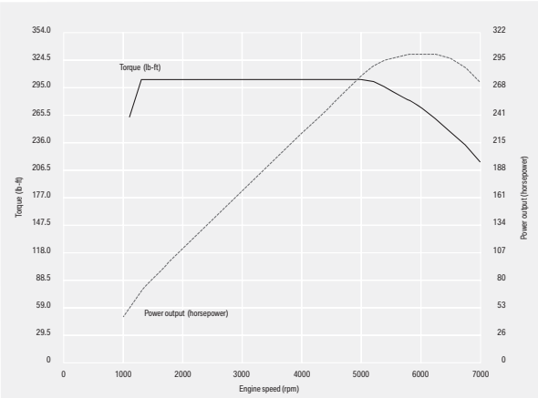
Portrait of an engineering masterpiece: the 335i s Advanced Turbo engine produces 300 horsepower at 5800 rpm, and quickly develops 300 lb-ft of torque at 1400 rpm, which continues without fading through to the 5000 rpm range. With such a broad range of powerful torque, you can enjoy smooth, robust acceleration in any gear, at any speed.
