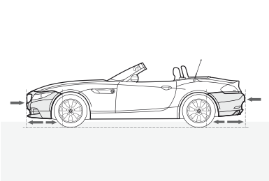
■ Impact-absorbing bumpers and compressible — crush tubes — front and rear help absorb the force of impact in collisions up to 9 mph, helping to minimize damage to the vehicle's body and simplifying repairs. Only at higher impact speeds do structural supports begin to deform, dissipating impact energy to help protect occupants.
