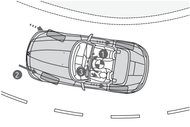
■ Cornering Brake Control (CBC) increases vehicle stability by proportioning the braking force while turning. When you brake in a turn, the pressure comes off the rear wheels, which (1) causes the vehicle to swerve inward (oversteer). Cornering Brake Control counteracts this action by asymmetrically adjusting brake pressure (2), creating stabilizing counter-torque (3) independently of the ABS system.
