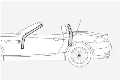
■ Z4 Roadster rollover protection consists of two steel roll bars behind the headrests; they are connected with a highly stable chassis crossbeam. The system is completed by a bar of high-strength tubular steel integrated into the windshield frame for maximum safety.
