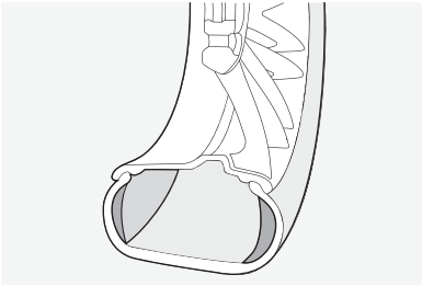
■ Run-flat tires allow speeds of up to 50 mph and travel from 30 to 150 miles after a loss of air pressure. 1 In situations that would normally result in a flat tire, reinforced sidewalls help prevent the tires from collapsing or loosening from the rim. In the event of a decline in tire pressure, the driver is warned by the Tire Pressure Monitor .
