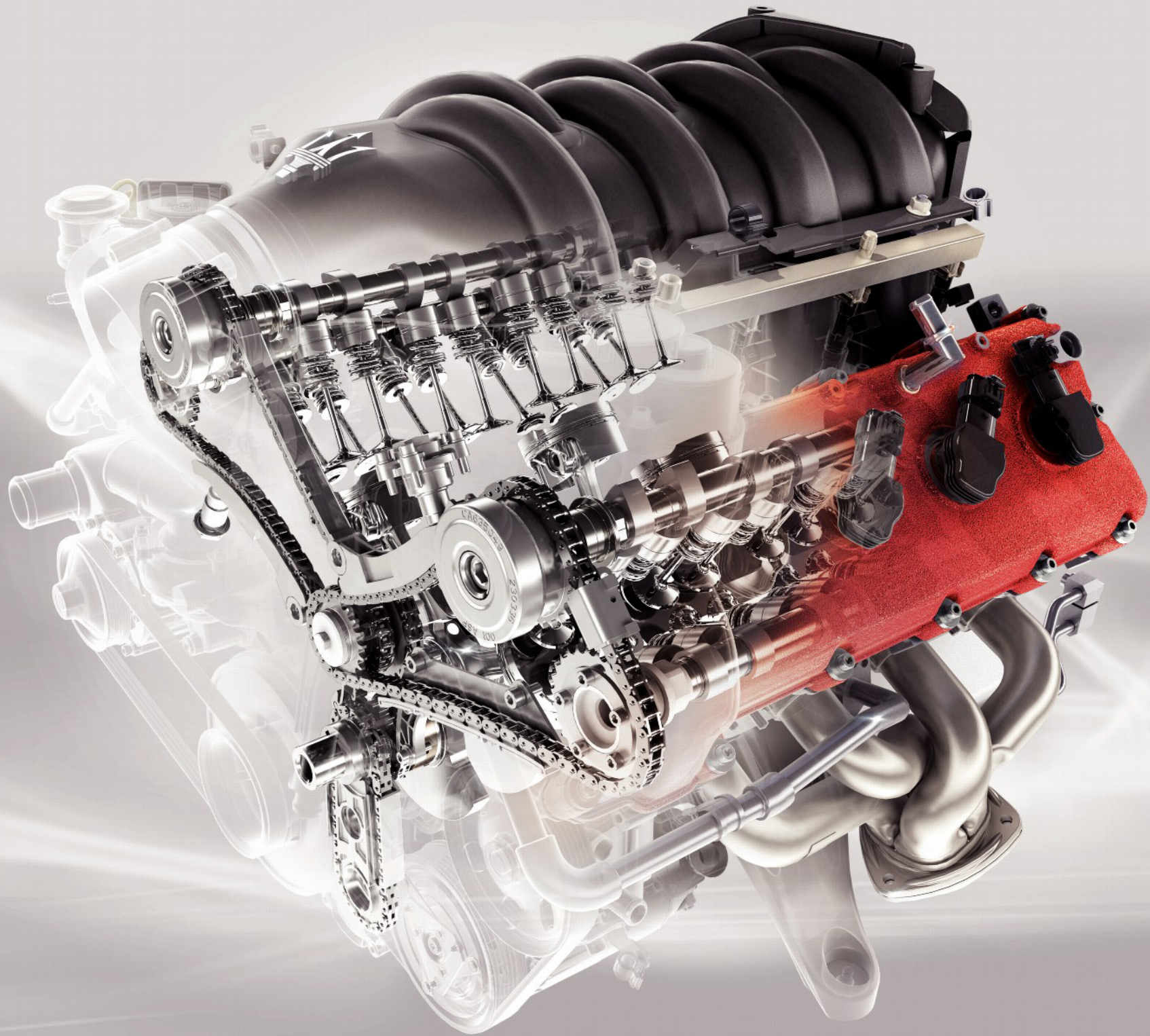
MASERATI V8 ENGINE 4.7 L
